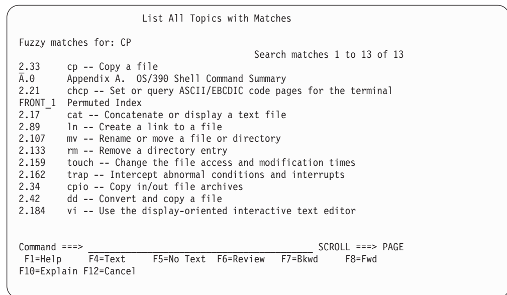
Figure 14. Sample Output from the Command OHELP cp
